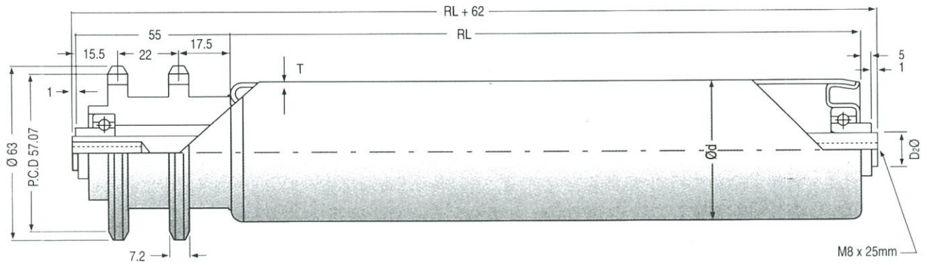
FIXED AND ACCUMULATIVE DRIVE CONVEYOR ROLLER C/W RS40 X 14T CHAIN SPROCKET
