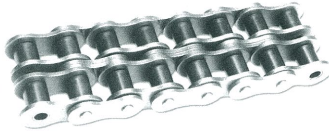
Double strand roller chain
